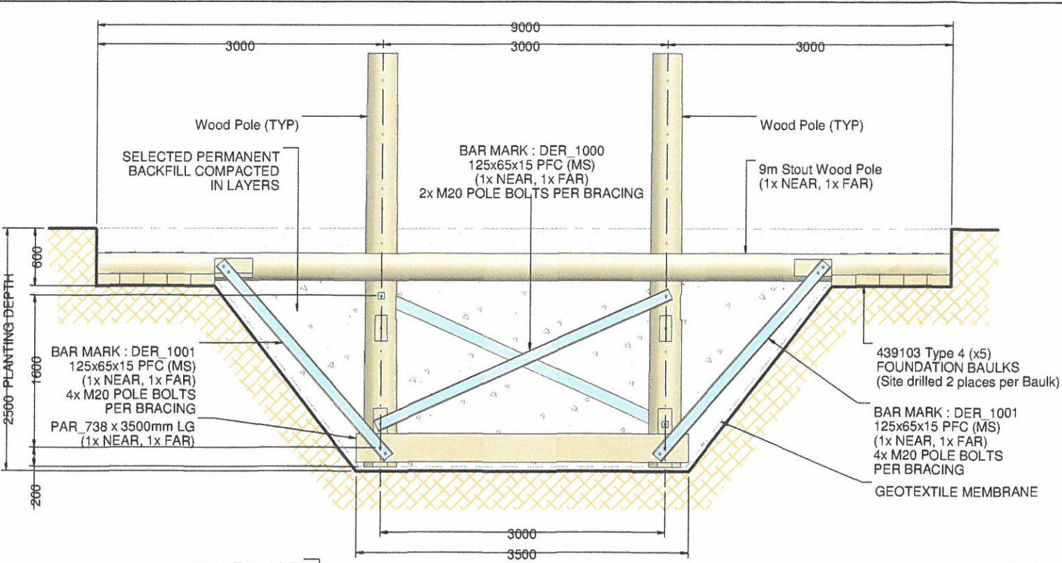
TRANSVERSE ELEVATION
